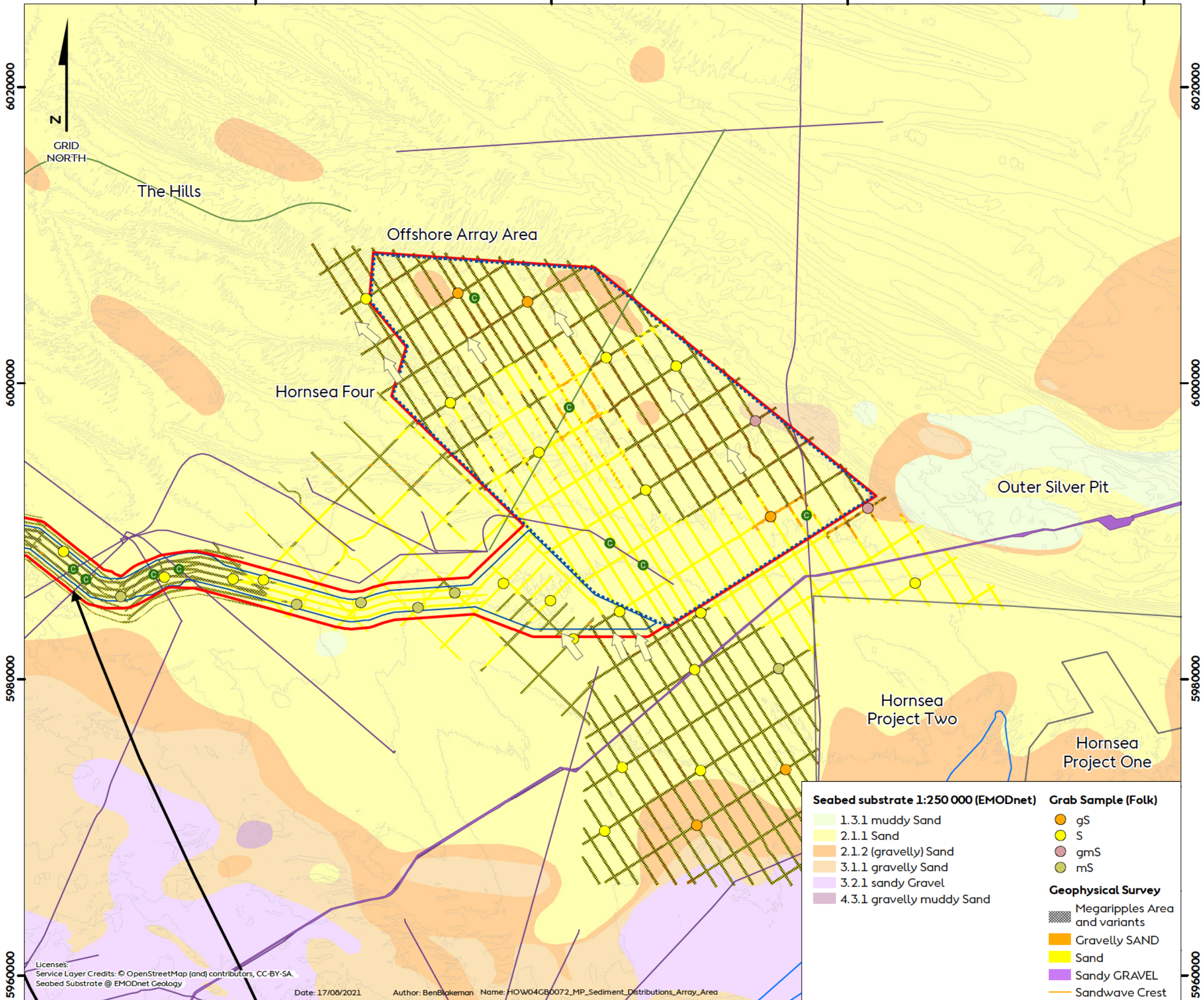
Figure 2 Sediment distributions across the offshore array study area
